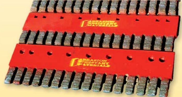
A.R.M.* 24H-M Normal Serrated – Patent granted.
