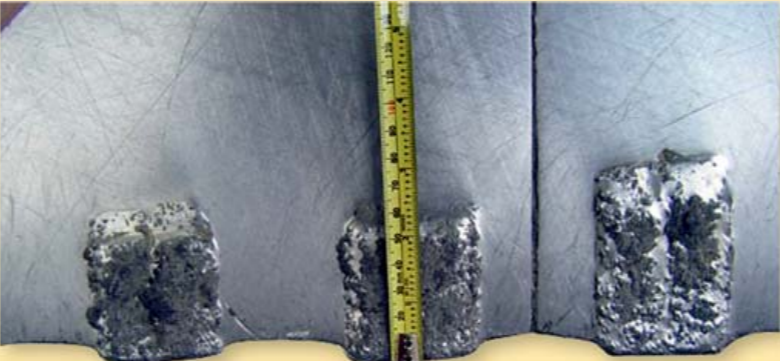
LH end wear rate A.R.M.* Semi-Serrated on 24M – after 800 hours.
