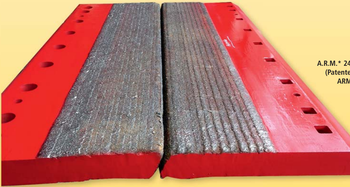
A.R.M.* Hardfaced 4ft Grader Edge for 16H & M Graders.
